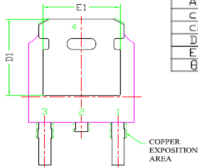
MATRIX L/F
